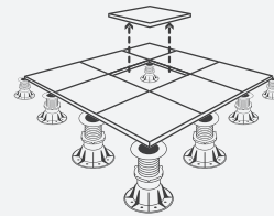
RAISED-ACCESS FLOATING FLOORING PAVIMENTO FLOTANTE REGISTRABLE
